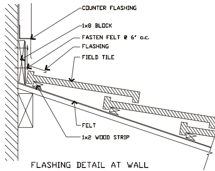
FLASHING DETAIL AT WALL
