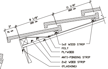
EAVE DETAIL
