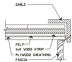
GABLE DETAIL
