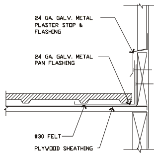
FLASHING DETAIL AT WALL
