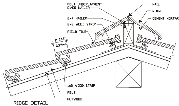
RIDGE DETAIL
