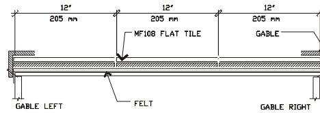
SPACE DETAIL
